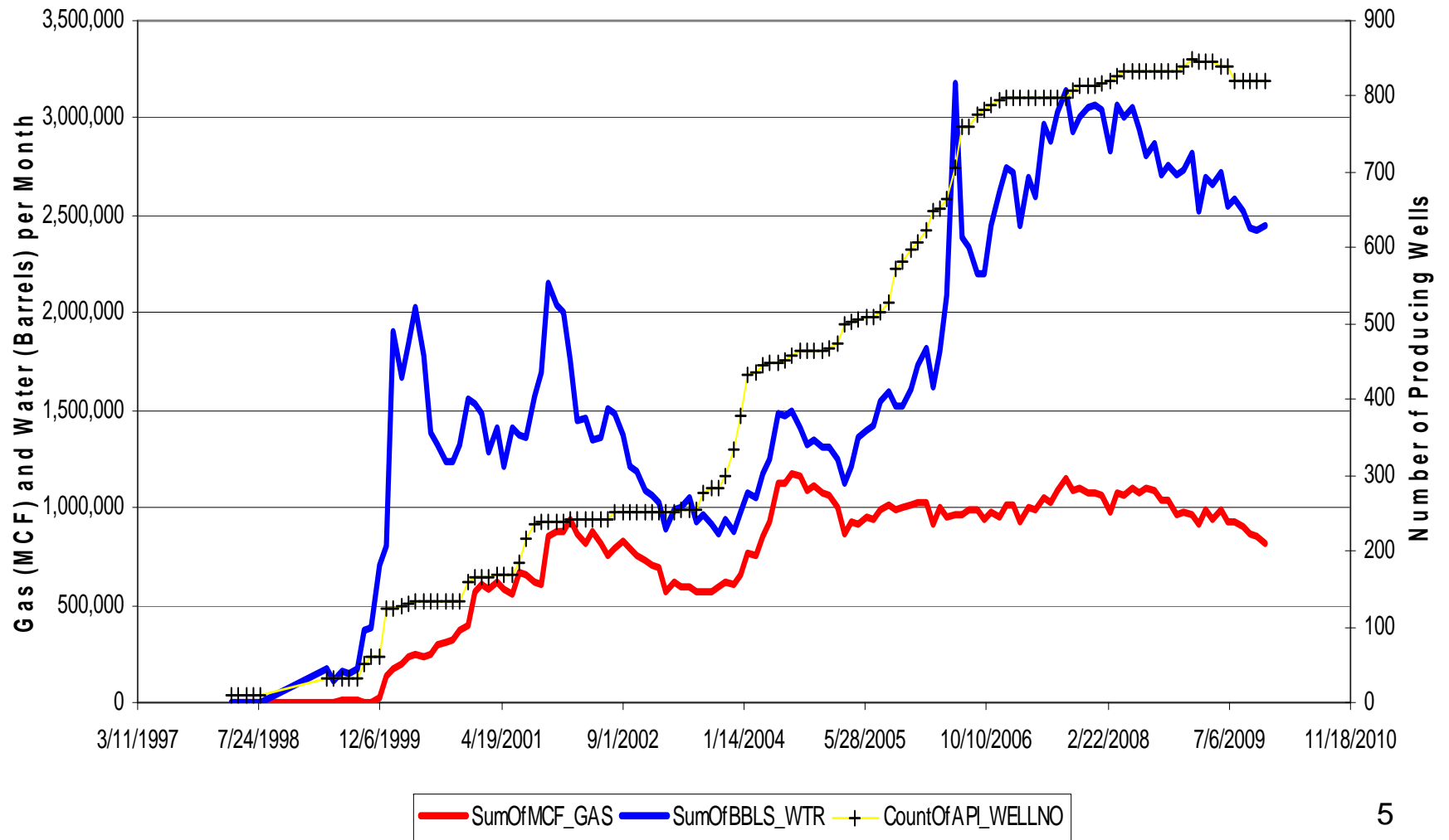
CX Field Monthly Production
