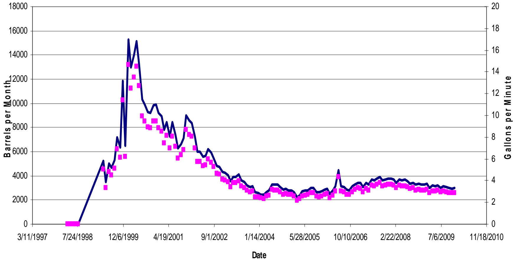
CX Field Average Water Production (Well)
