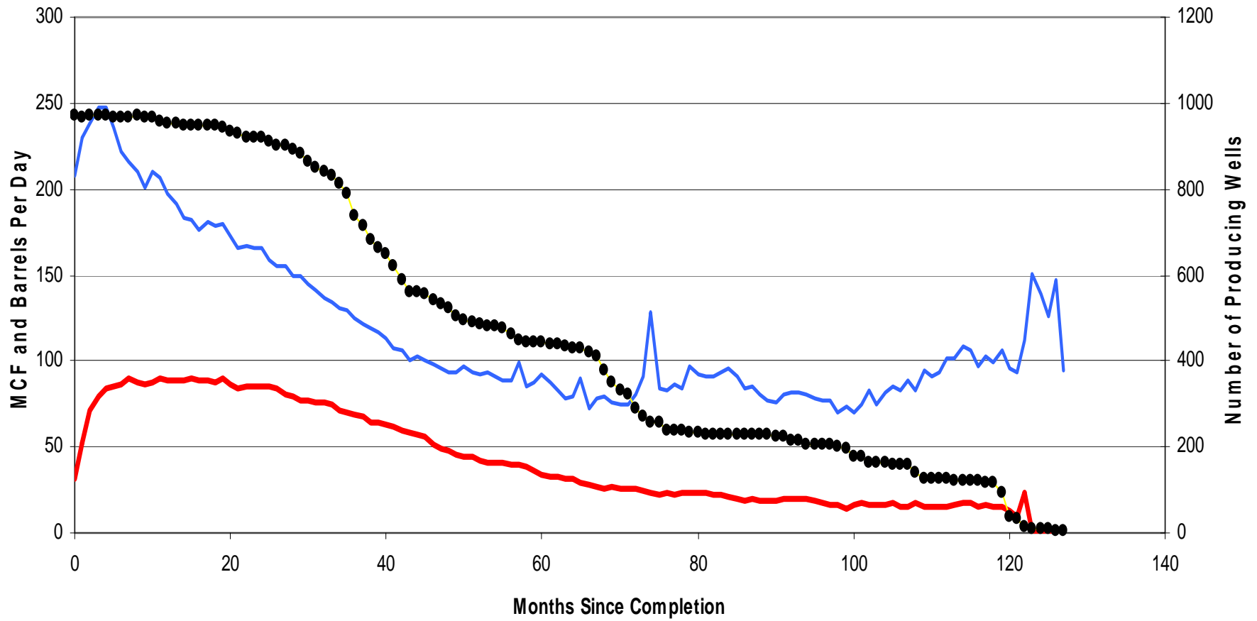
Average CBM Well Production
