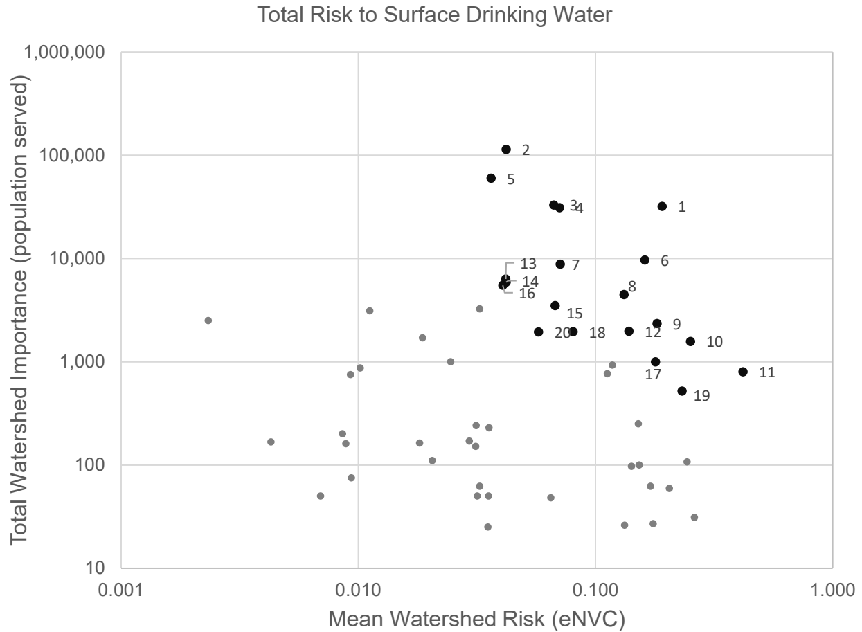
Figure B.2. Total risk to surface drinking water in Montana. The top 20 most at-risk systems are numbered by rank (See Table B.2).
