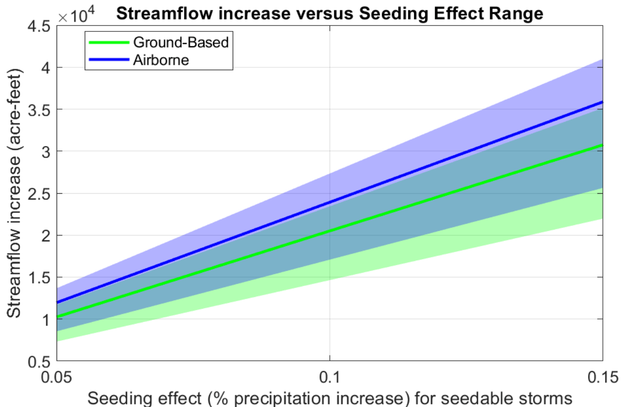
Figure 5.24. Estimates of streamflow increases into the study area using 5, 10, and 15% levels of seasonal seeding effects for seedable storms. The streamflow calculations include adjustments to relate the seeding effects to total assessment area precipitation, which requires an estimate of assessment area seeding coverage. The range of streamflow estimates for the various levels of area coverage (50–80%) are denoted by the different color-shaded areas. The 70% area coverage (solid lines within the color-shaded areas) are used for streamflow estimates assumed in the benefit/cost calculations. Ground-based seeding is indicated by green colors, and airborne by blue.
