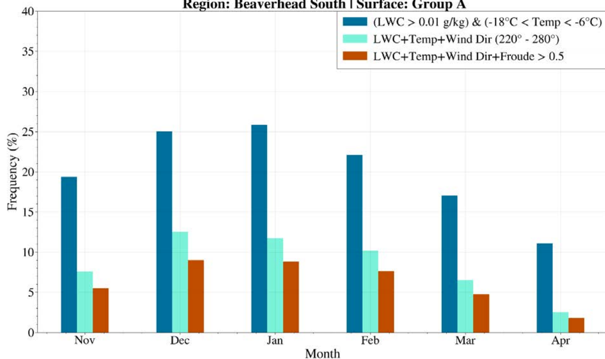
Ground Monthly Seeding Frequency CONUS404 Current Climate Region: Beaverhead South | Surface: Group A
