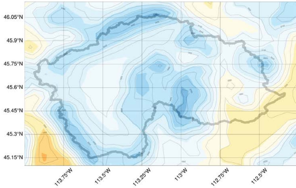
CONUS404 Current Climate Ground Temperature Average (February)
