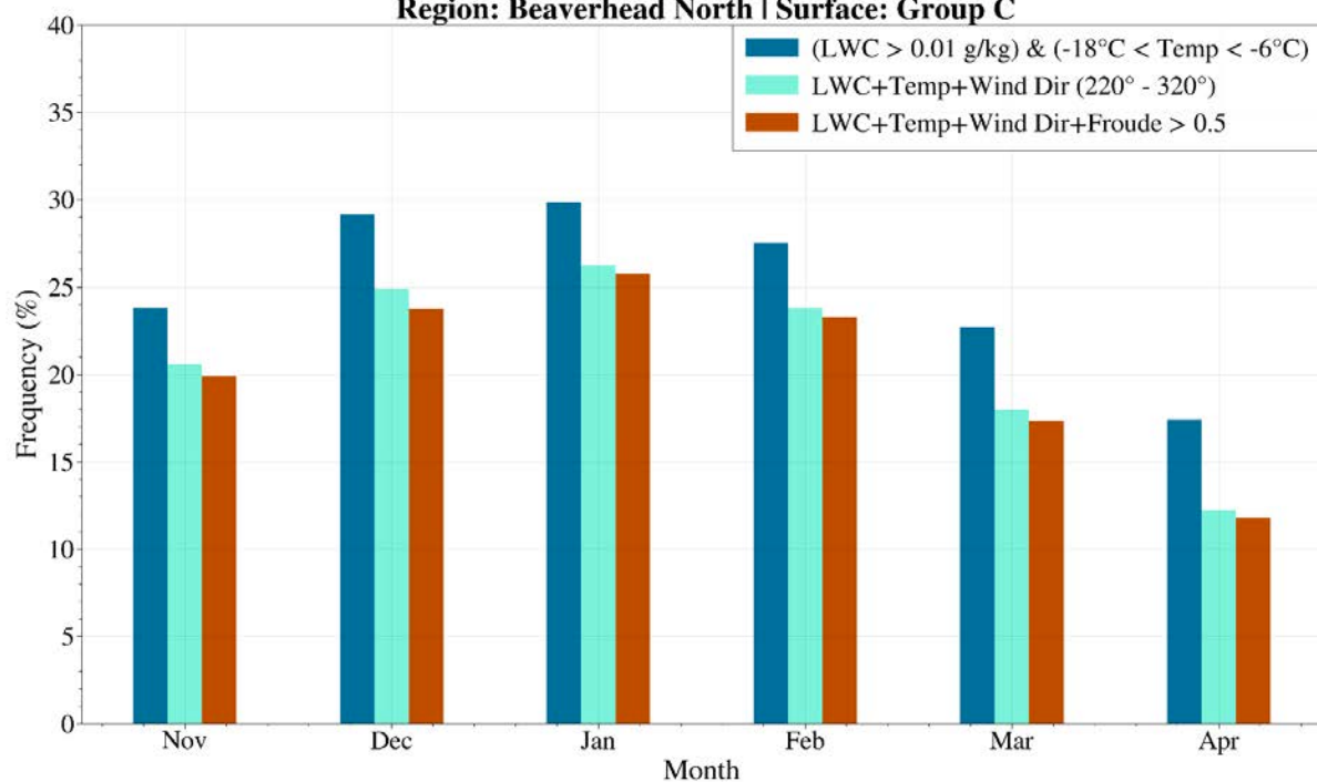
Ground Monthly Seeding Frequency CONUS404 Current Climate Region: Beaverhead North | Surface: Group C
