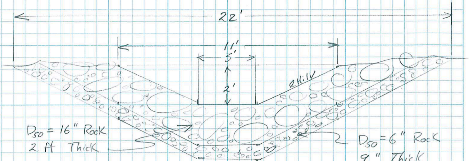
10% Slope Channel Section 1" = 3'
