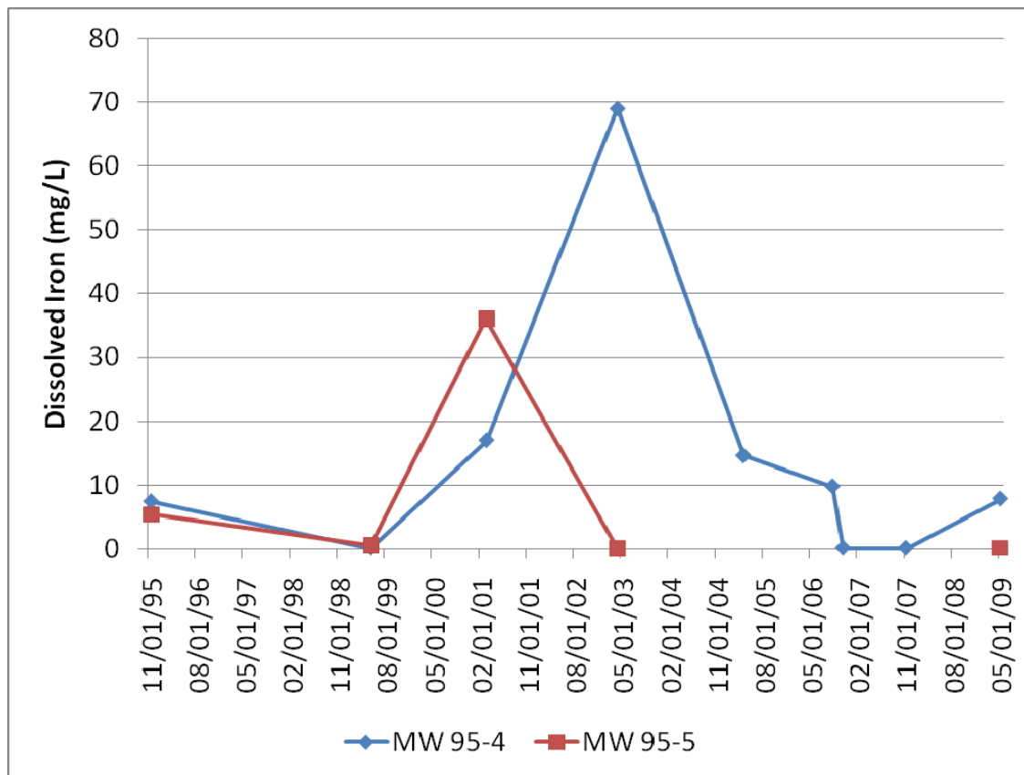
Figure 1 – Variations in dissolved iron concentrations with time for wells MW 95-4 and MW 95-5.
