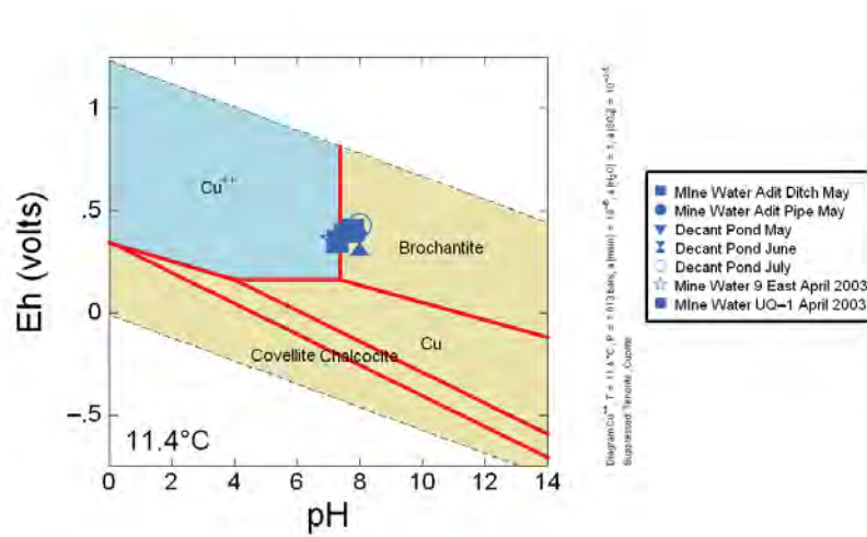
FIGURE 10. EH-PH DIAGRAM FOR COPPER (ACTIVITY = 10^{-6} ) WITH SULFATE (ACTIVITY = 10^{-3.5} )
