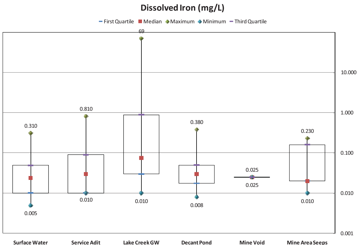
Figure 5 – Comparison of dissolved iron concentrations between the mine area surface water (seeps) and the other waters (note the logarithmic scale).
