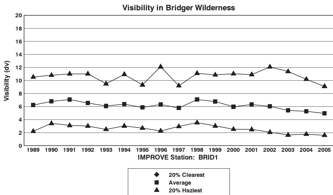
Figure 3-3. Visibility in the Badlands and Bridger Wilderness Area.
