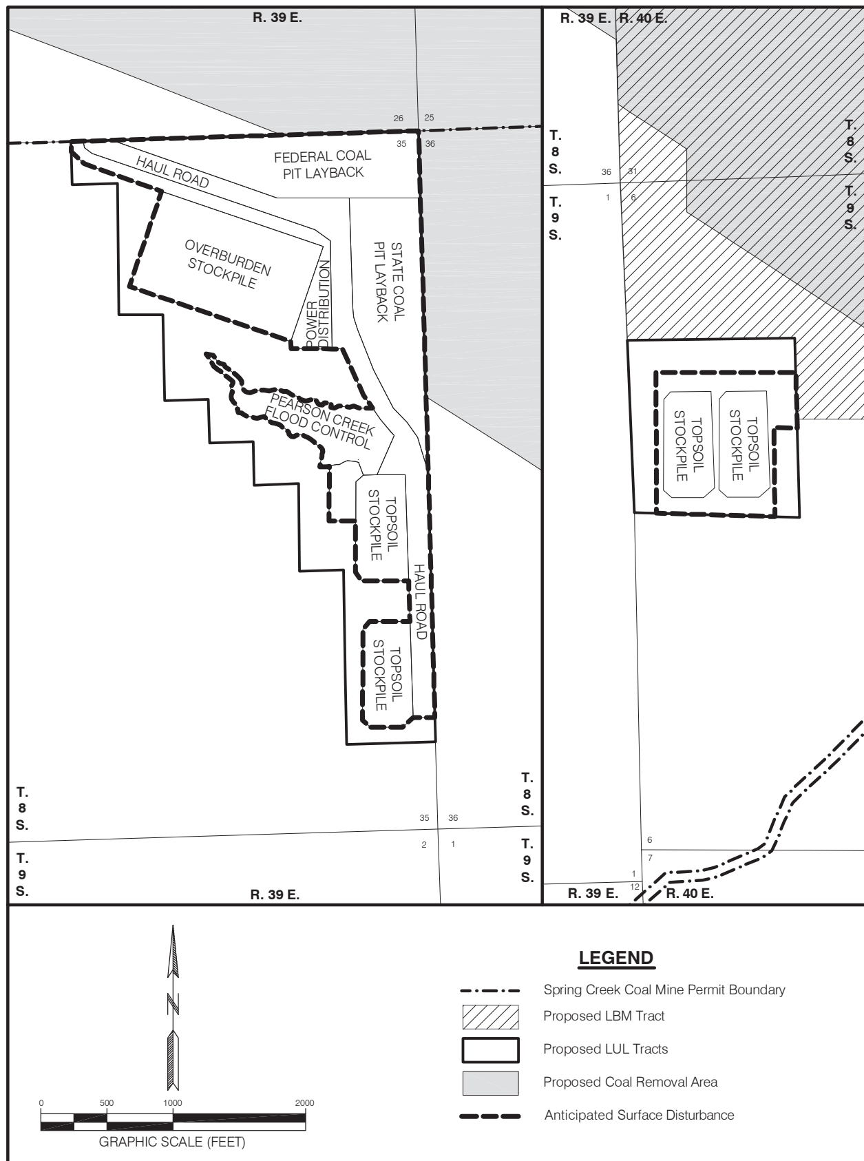
Figure 2-3. Initial Surface Disturbance Associated With the LUL Tracts.
