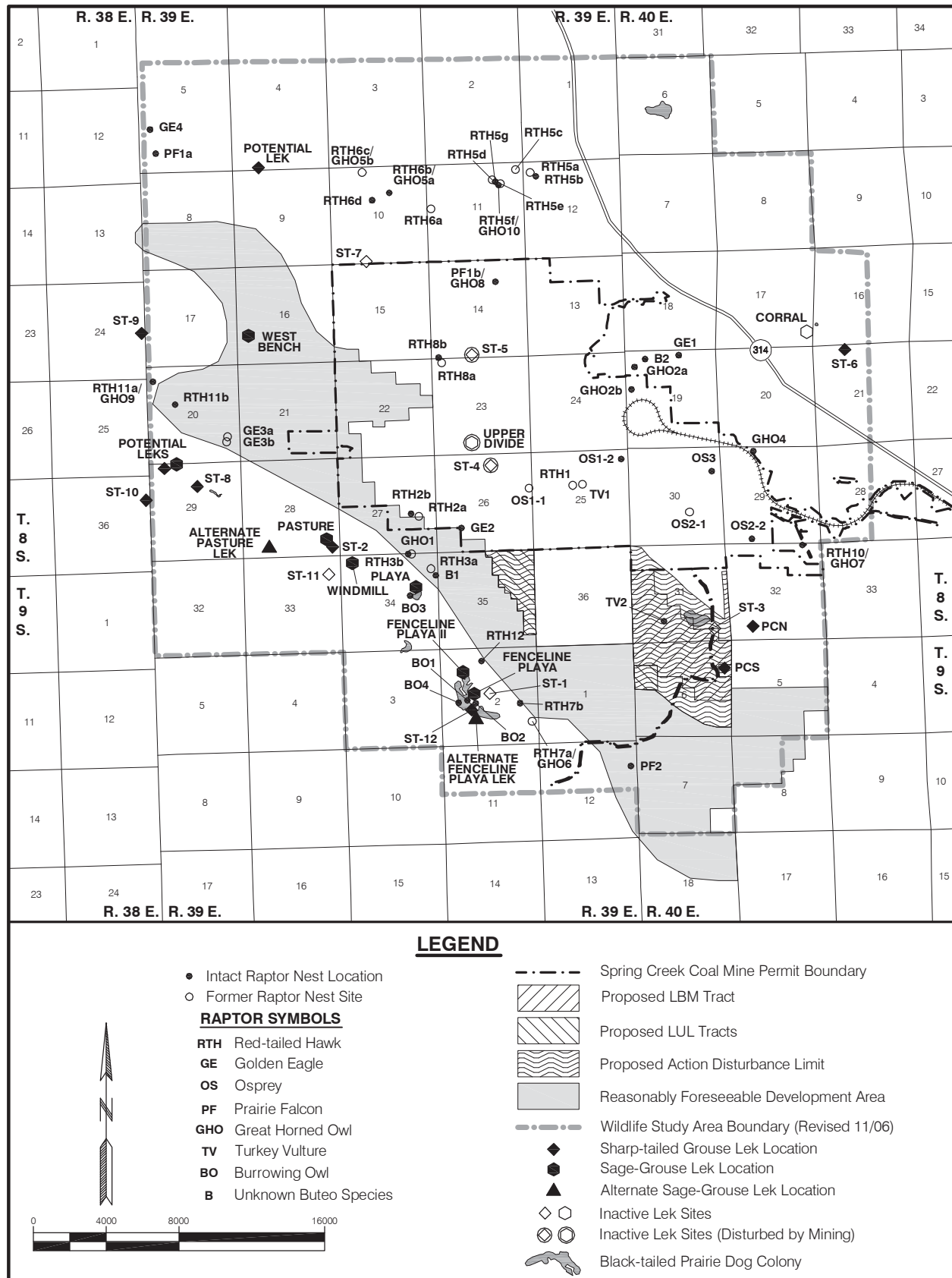
Figure 3-9. Wildlife Use Associated with the Proposed LBM and LUL Tracts and the Spring Creek Coal Mine Area.
