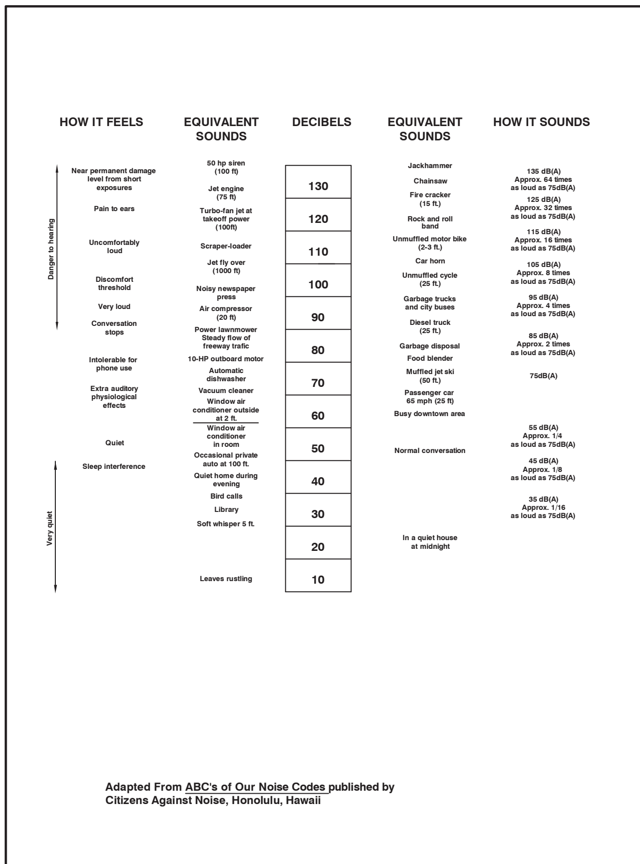
Figure 3-13. Relationship Between A-Scale Decibel Readings and Sounds of Daily Life.
