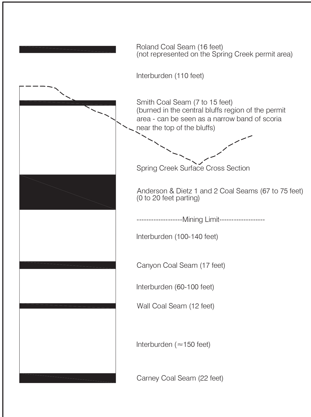
Figure 3-2. Generalized Stratigraphic Cross Section Through the Spring Creek Coal Mine Area.
