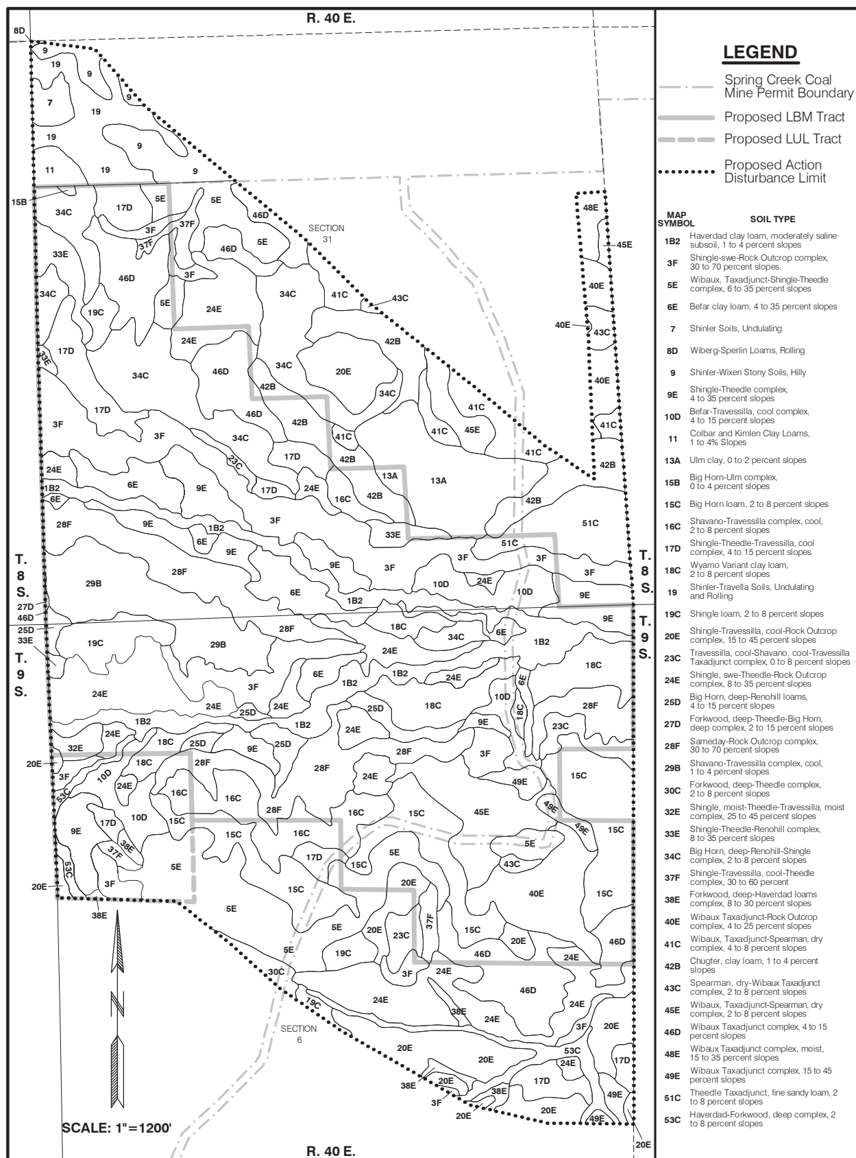
Figure 3-5. Soil Mapping Units Within the Proposed Action Disturbance Limit.
