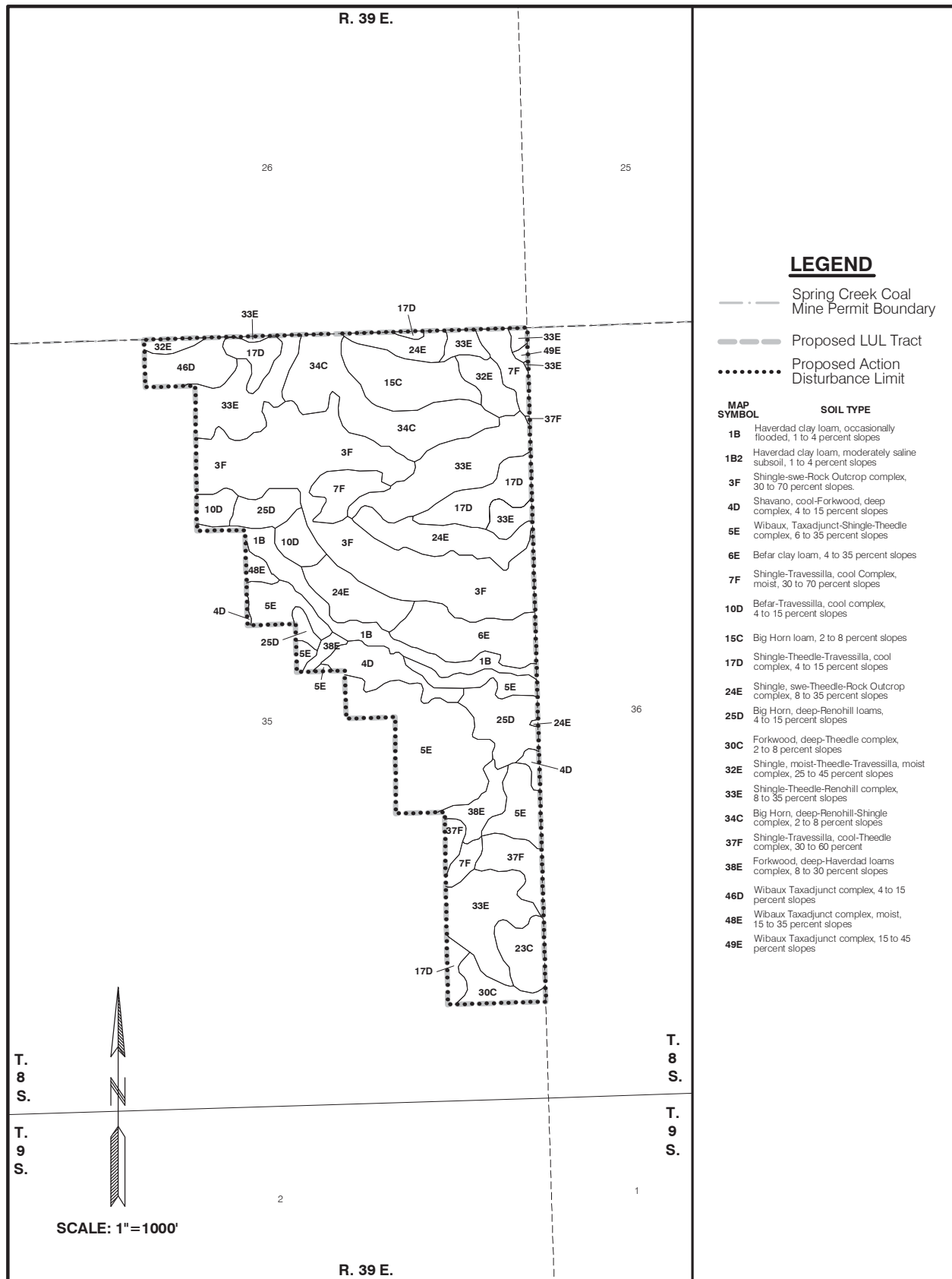
Figure 3-6. Soil Mapping Units Within the Proposed Action Disturbance Limit.
