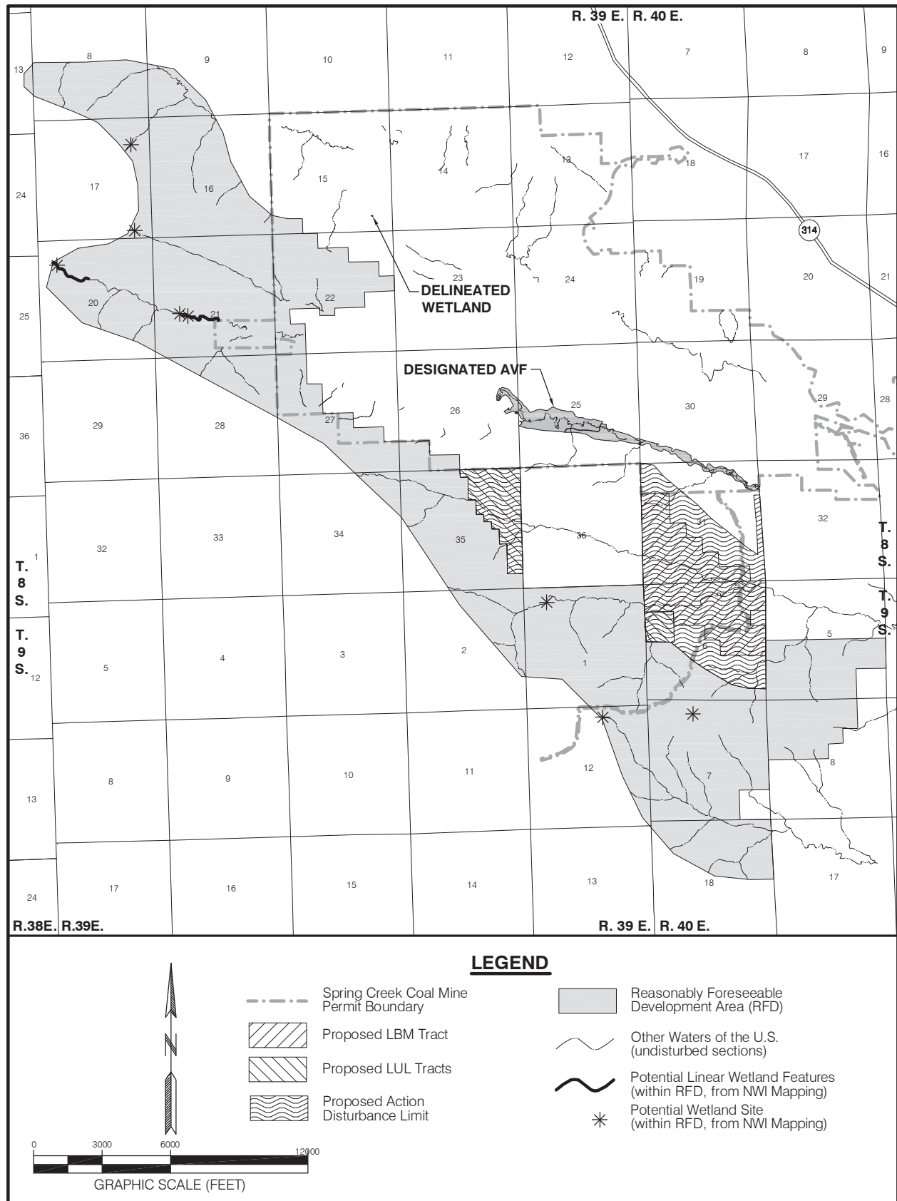
Figure 3-4. Delineated Wetlands and Designated AVF's Associated with the Proposed LBM and LUL Tracts and RFD Area.
